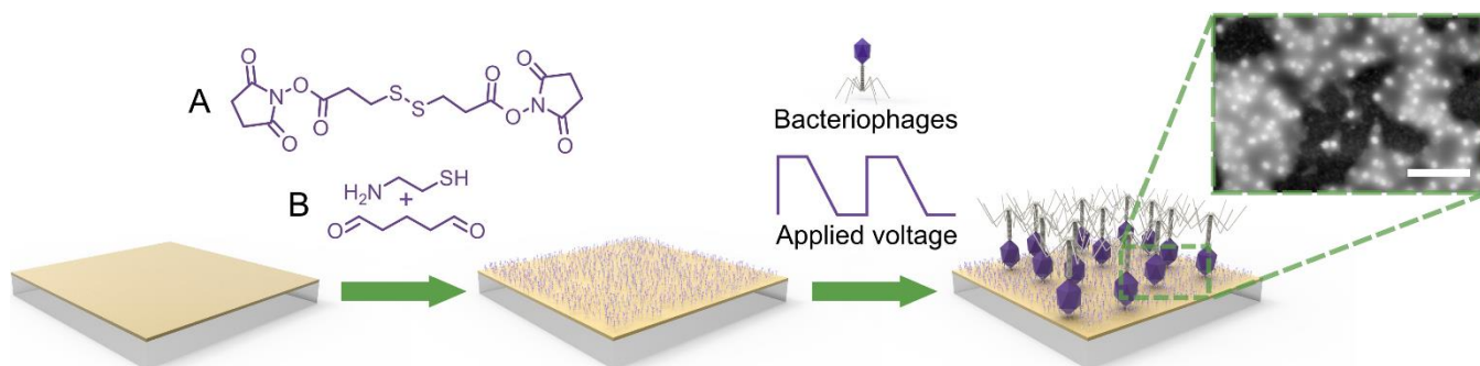
Figure 1. Scheme for fabricating dense sensing layers of ordered phages. At first gold surface was modified with (A) dithiobis(succinimidyl propionate) (DTSP) or (B) cysteamine and subsequently glutaraldehyde. Second step consisted of deposition of phages in the alternating electric field. Magnification box shows the atomic force microscopy image of the densely packed sensing layer of ordered bacteriophages. Scale bar corresponds to 1 μm. As the third step of sensing element
